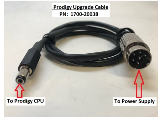
12VDC adapter cable #1700-20038
