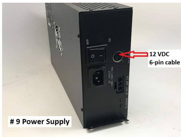
#9 Power supply
